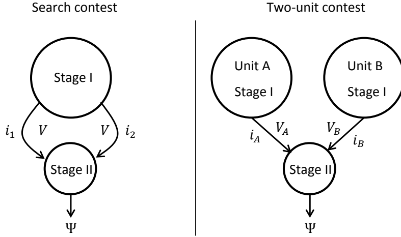
Figure 2: Search and two-unit contest
