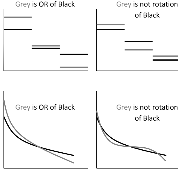
Figure 1: Class I and II rotations
